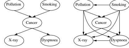
Figure 3: Left: Causal graph of Cancer dataset. Right: GPT-3.5's estimated causal graph. GPT-3.5 gets causal order correct at the cost of higher SHD score Here D_{top} = 0 and SHD = 6
