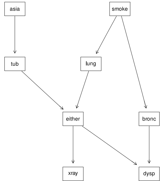
Figure A4: Asia Bayesian network. Abbreviations/Descriptions: asia=visit to Asia/visiting Asian countries with high exposure to pollutants, smoke=smoking habit, tub=tuberculosis, lung=lung cancer, either=either tuberculosis or lung cancer, bronc=bronchitis, dysp=dyspnoea, xray=getting positive xray result.
